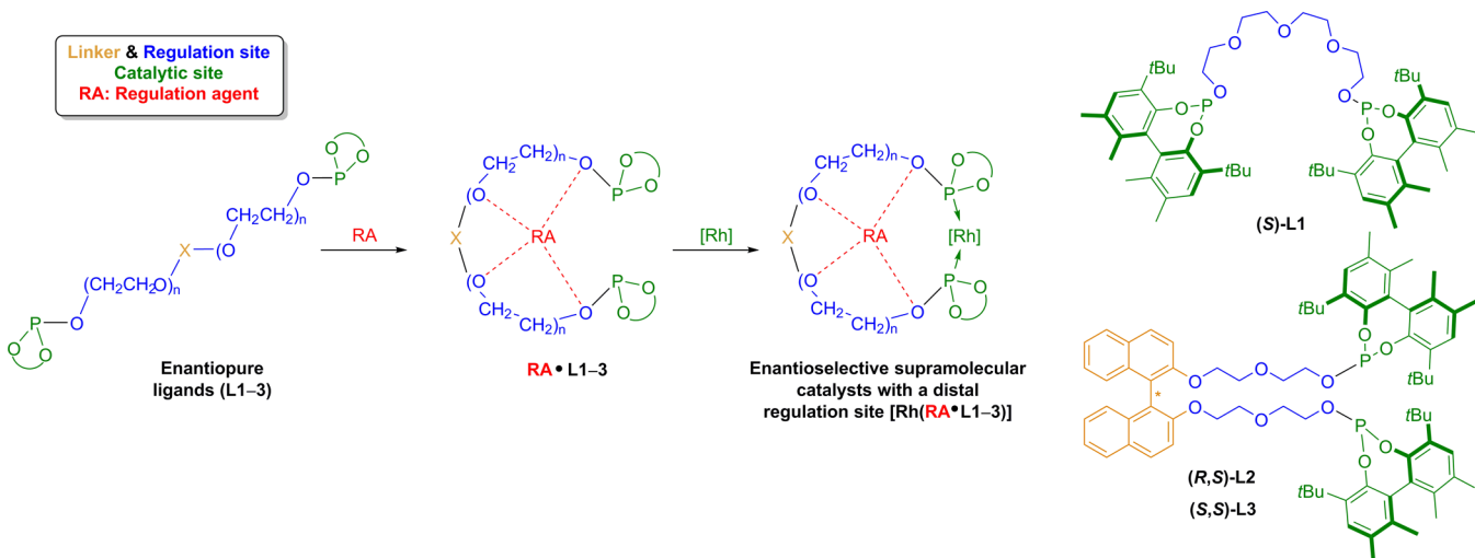
Scheme 2. AHF of Compounds 1a–e Mediated by Supramolecularly Regulated Ligands L1–3
